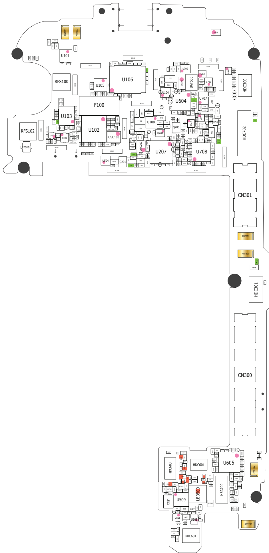
Top PCB Layout
